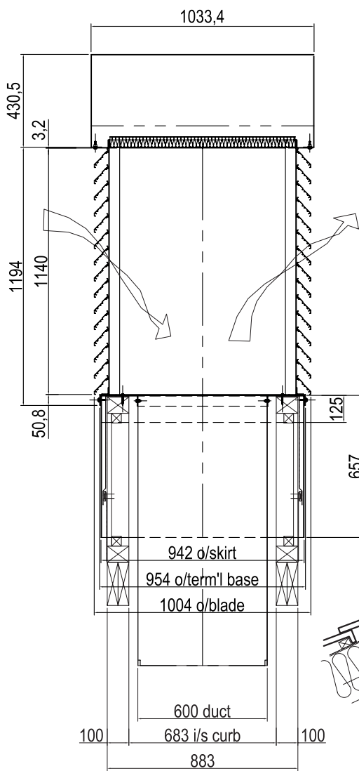
Sectional Front Elevation
