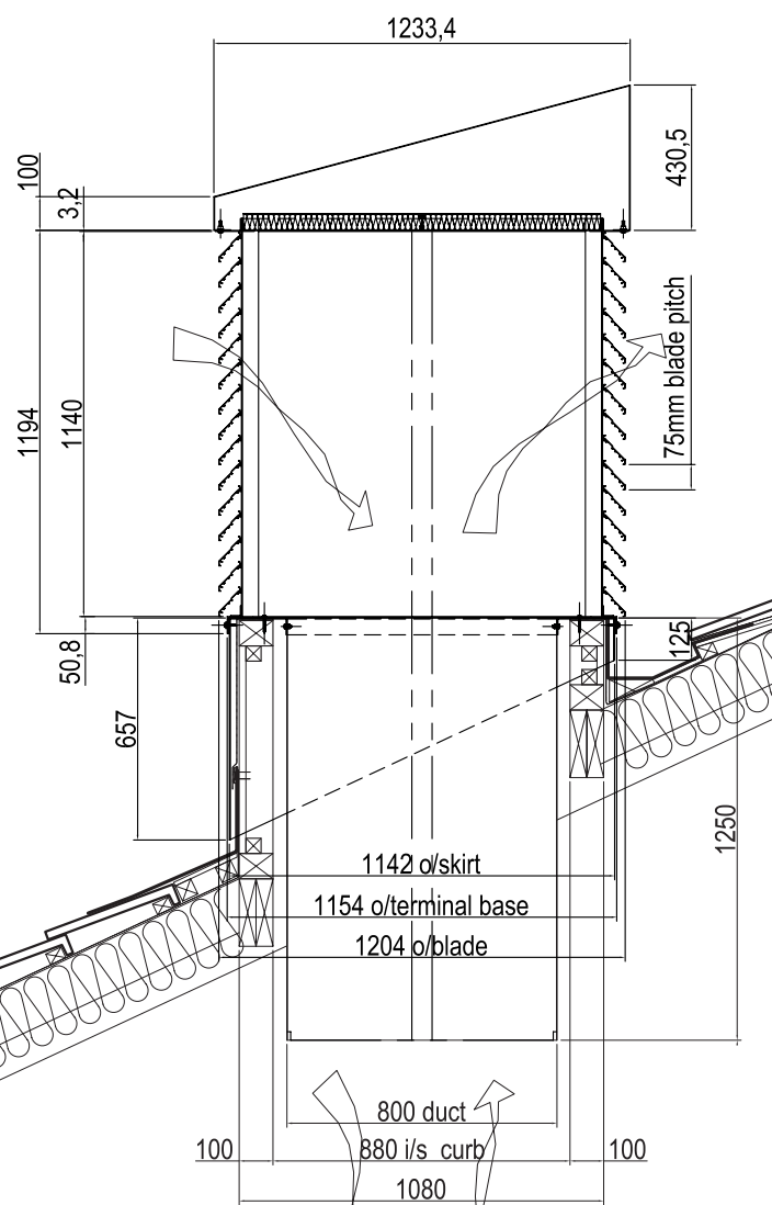
Sectional Side Elevation
