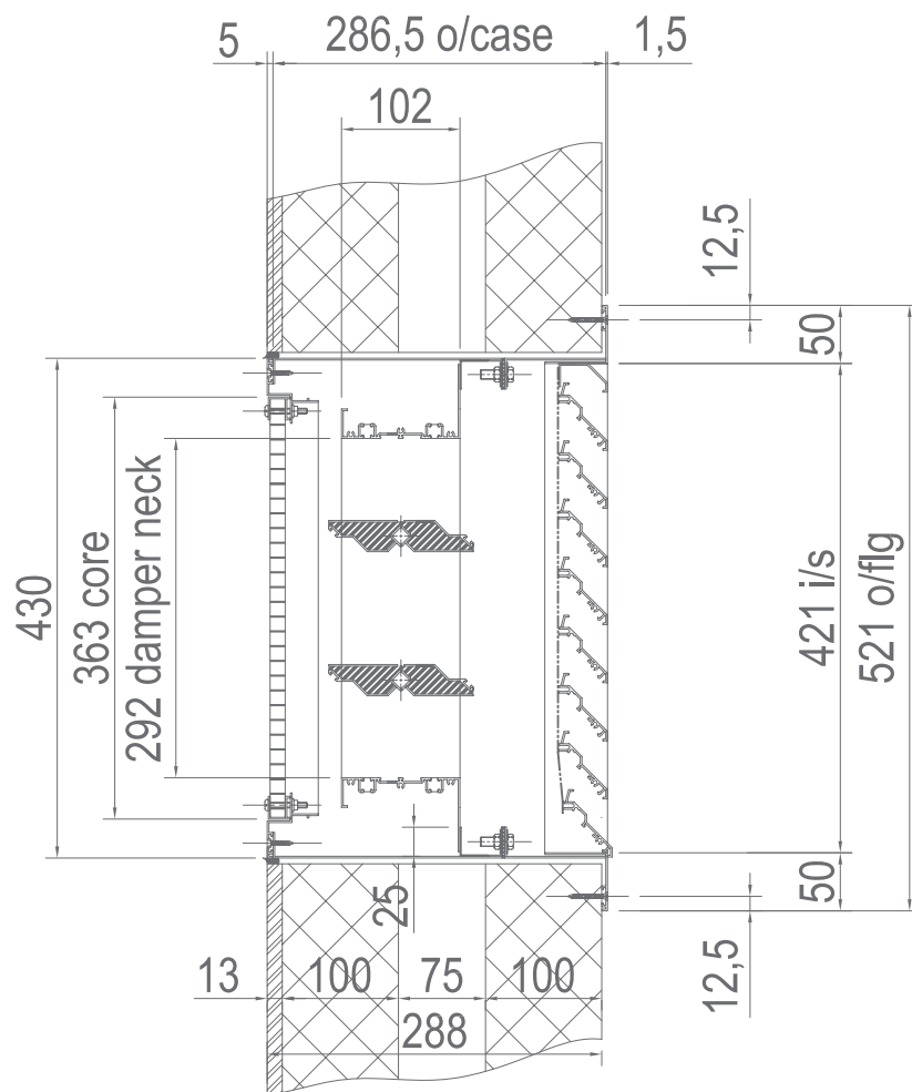
Sectional Plan View
